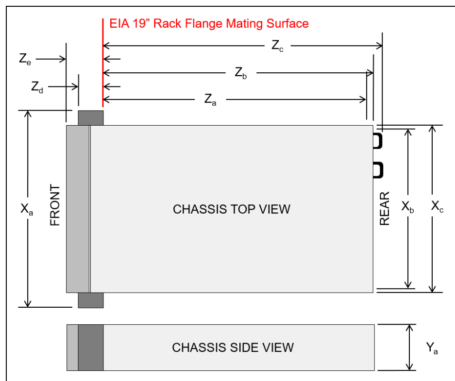
Figure 12. Server dimensions
